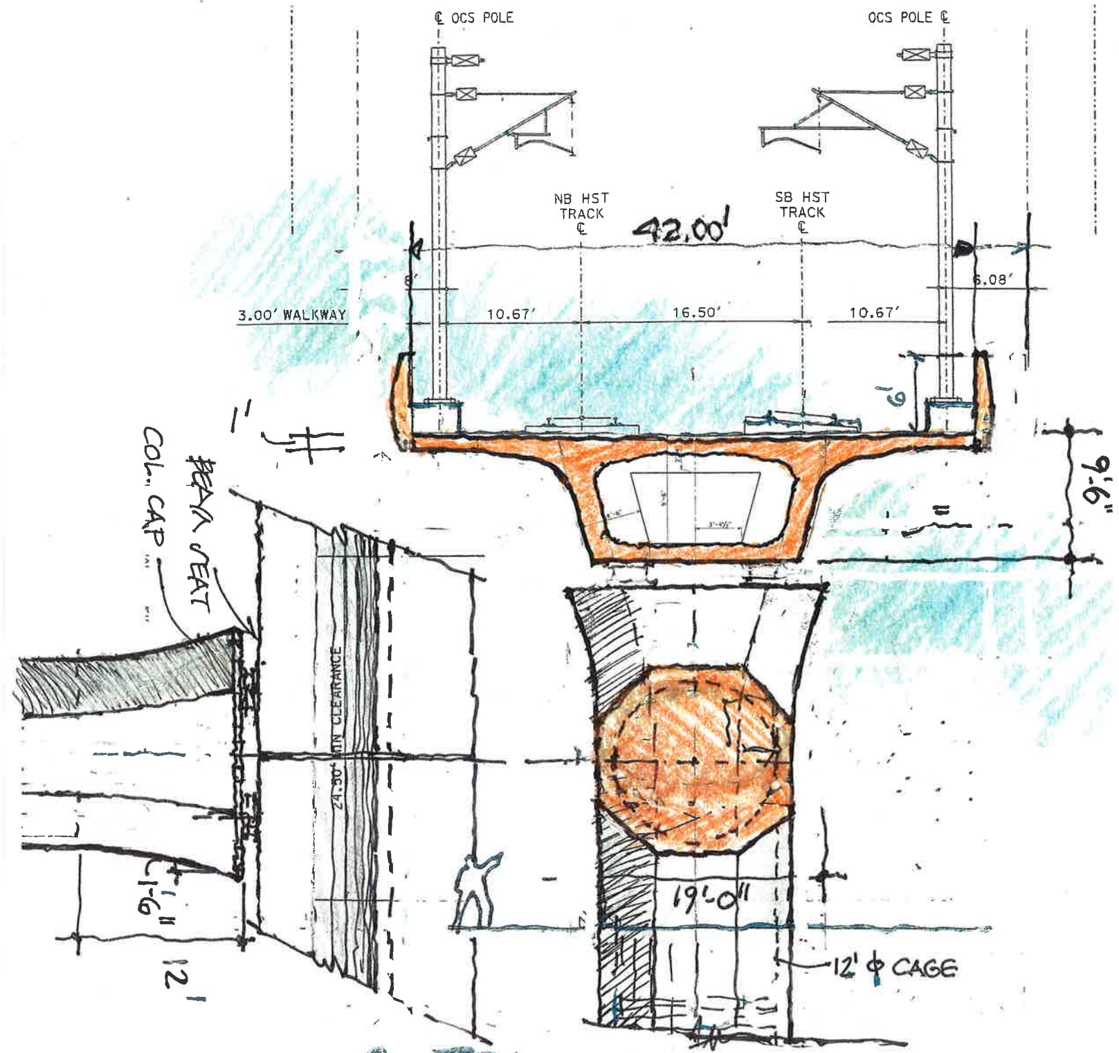
2-TRA CURVED GIRDER
