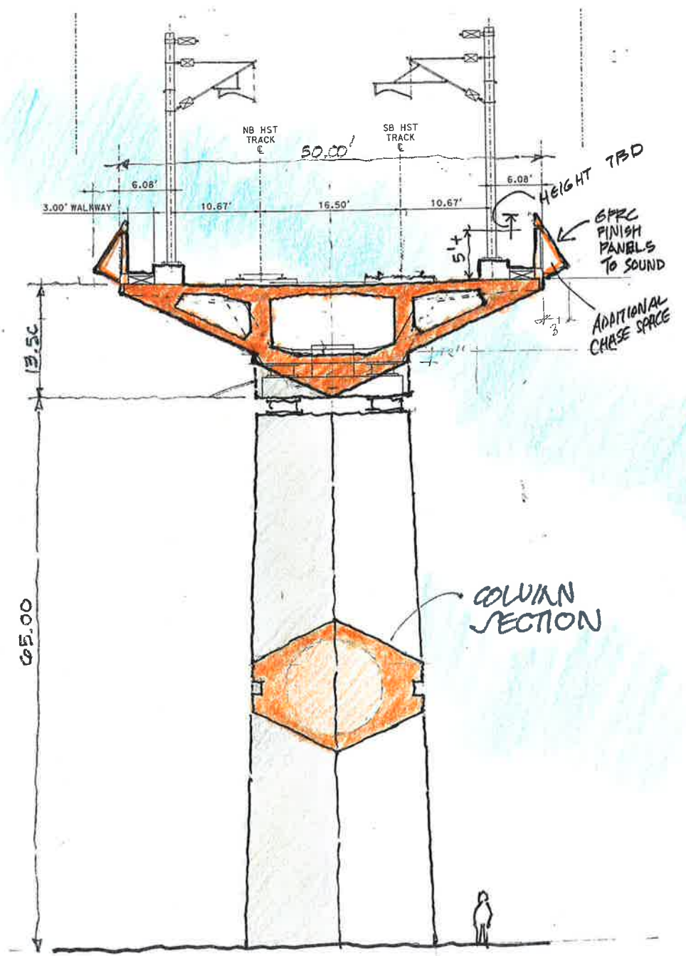
TALL COLUMN - TWO TRACK DELTA GIRDER
