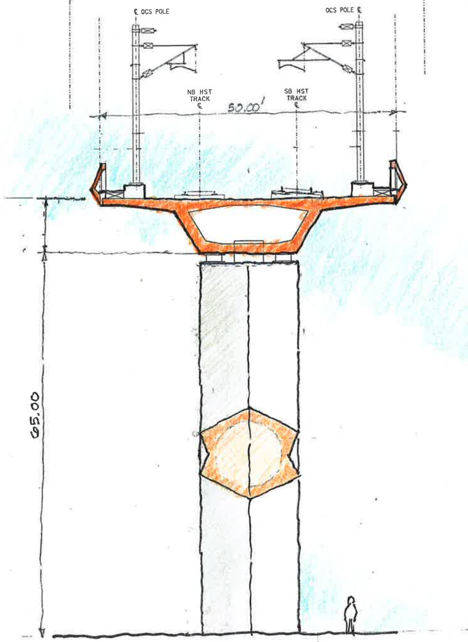
TALL COLUMN - TWO TRACK STD GIRDER
