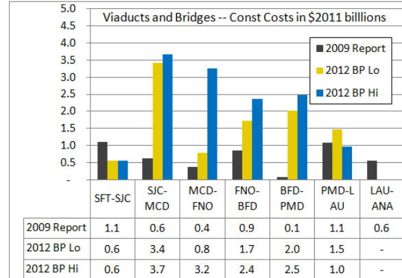
Exhibit 10 Viaduct and Bridges Construction Costs (2011$ billions)
