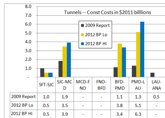
Tunnels Construction Costs (2011$ billions)
