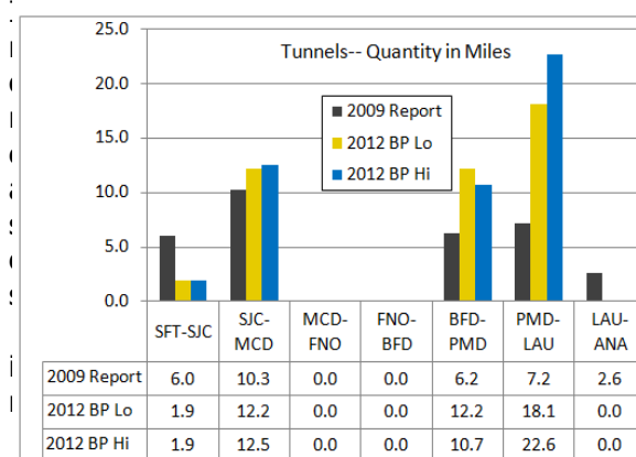
Tunnels Quantities in Miles
