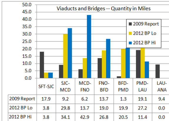
Exhibit 9 Viaduct and Bridges Quantities in Miles
